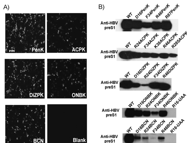
Figure 1. Encoding UAAs in human hepatocytes by the Pyl-based system. A) Huh-7 cells transfected with plasmids encoding the PylRS-tRNA Pyl CUA pair and GFP-Y40-TAG with and without the indicated Pyl analogues (1 mM final concentration) were visualized by fluorescent microscopy. All images are in the same scale (scale bar: 100 μm). B) Western blotting analysis using the mouse monoclonal antibody-2D3 that specifically recognizes residues 19–33 of the Pre S1 domain on L protein. The expression of HBV L protein with the Pyl analogues at indicated sites in Huh-7 cells was detected by 2D3.
